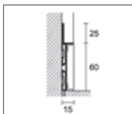
88/6 + 88/16SF aluminium insert
