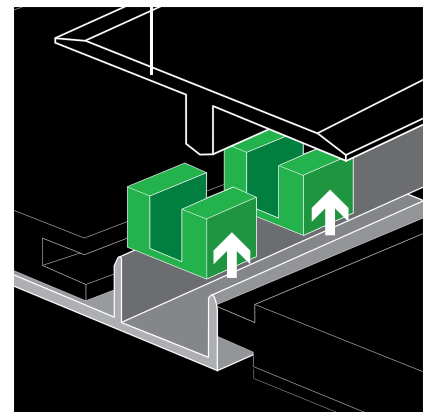
insert the clips in the top profile
