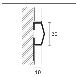
AVK/1 chromium-plated brass
