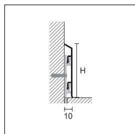
95/7 silver anodised aluminium
