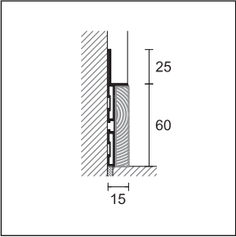
88/16SF solid wood insert
