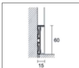
87/6 + 88/16SF aluminium insert
