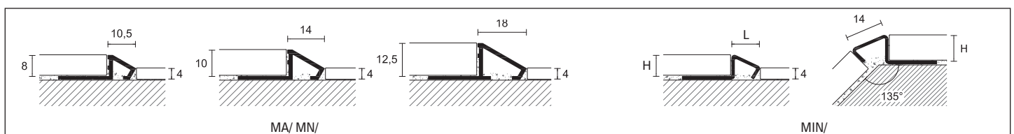
MIN/10 polished stainless steel AISI 304 DIN 1.4301
