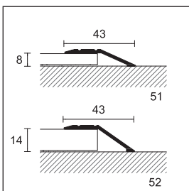
51/A gold anodised aluminium
