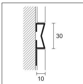
AVK/2 chromium-plated brass
