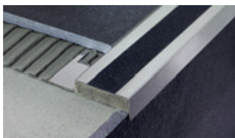
SIX/10 satin stainless steel AISI 304 - DIN 1.4301 + black slip-resistant 25 mm
