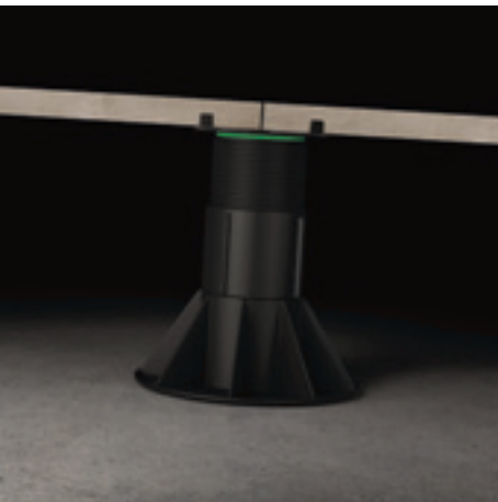
with Perfect Ring, the support is fixed
