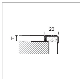
SMA/4,5 natural aluminium
