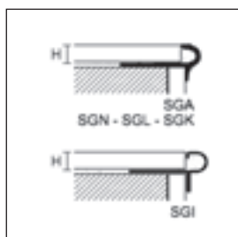
SGI/11 polished stainless steel AISI 304 DIN 1.4301
