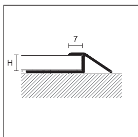
GF/710 silver anodised aluminium
