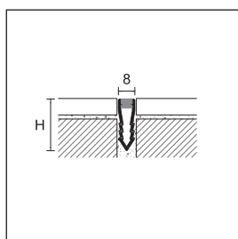
NF/45 co-extruded PVC grey + grey RAL 7035
