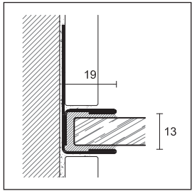
GPS2/19 satin stainless steel AISI 304 DIN 1.4301
