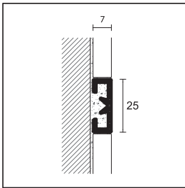
LDS/20 bright satin silver aluminium
