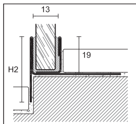
GPS1/DX/19 satin stainless steel AISI 304 DIN 1.4301
