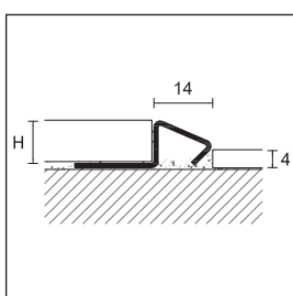
MIN/10 application for floors of different height
