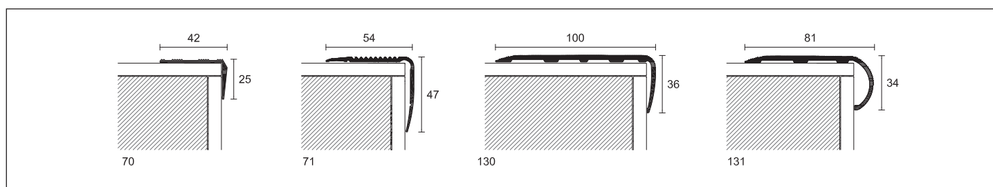
71/SF silver anodised aluminium
