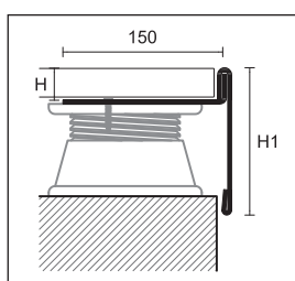
CPLB + CPLV/60 ash grey RAL 7038 colour-coated aluminium
