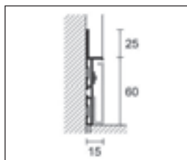
88/6 + 88/16L/A aluminium insert for LED light
