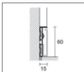
87/6 + 88/16L/A aluminium insert for LED light
