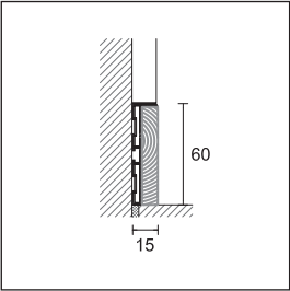
87/6 + 88/16SF solid wood insert
