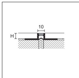
NL/10 co-extruded PVC grey + grey RAL 7035
