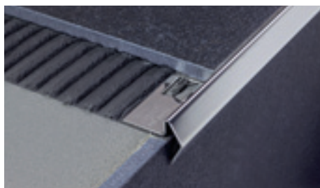
SI/10 polished stainless steel AISI 304 - DIN 1.4301
