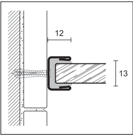
GPS14/12 satin stainless steel AISI 304 DIN 1.4301
