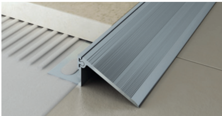
NZS/B/12 + NZS/S2 silver anodised aluminium
