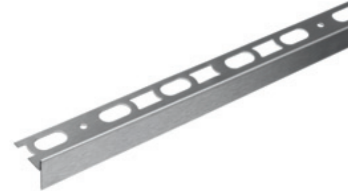
GPS3/DX/10 satin stainless steel AISI 304 DIN 1.4301
