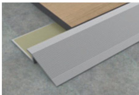
PBA/5A silver anodised aluminium
