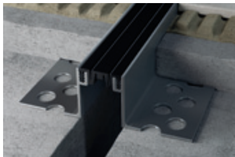
PBE/30 natural aluminium + striated black rubber
